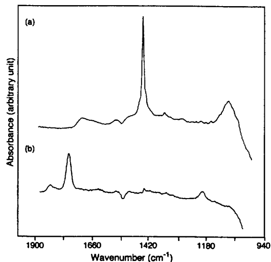
Figure 5. Transmission FT-IR spectra of LB films ( 15 \times 2 layers) of 2C_{18}DAE/IA-EVE on CaF_2 plates: (a) as-deposited. (b) heat-treated at 180^\circ C for 6 h under vacuum.
