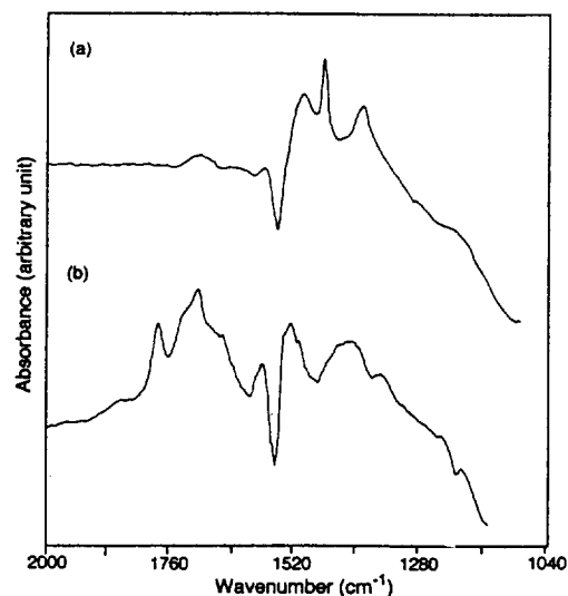
Figure 4. Transmission FT-IR spectra of LB films ( 1 \times 2 layers) of 2C_{18}DAE/IA-BVE/PAA on CaF_2 plates: (a) as-deposited film. (b) heat-treated film at 180 \text{ }^\circ\text{C} for 6 h under vacuum.
