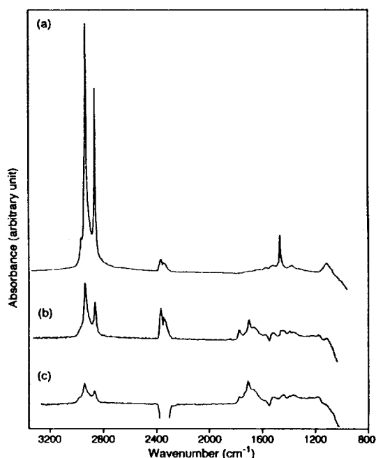
Figure 6. Transmission FT-IR spectra of LB films ( 15 \times 2 layers) of 2C_{18}DAE/IA-EVE/PAA on CaF_2 plates: (a) as-deposited. (b) heat-treated at 180^\circ C for 6 h under vacuum. (c) extracted by chloroform after immersion in aq. NaCl followed heat treatment.
