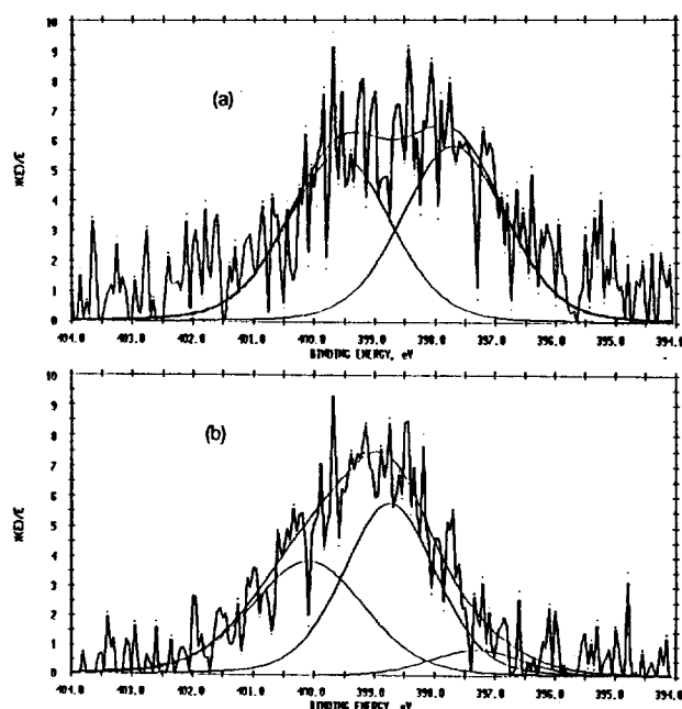
Figure 7. XPS spectra of the N_{1s} region of a 12 layer LB film of 2C_{18}DAE/IA-BVE/PAA on a fluorocarbon membrane filter (FP-010): (a) as-deposited. (b) after heat treatment at 180^\circ C for 6 h under vacuum. The charging shift was not corrected.
