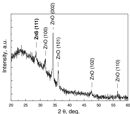
Fig. 5 XRD pattern of the sample obtained from solution containing ZnCl 2 and thiocarbamide (Zn:tu = 1:0.5), [Zn] = 0.1 mol. Diffraction was recorded using parallel beams
